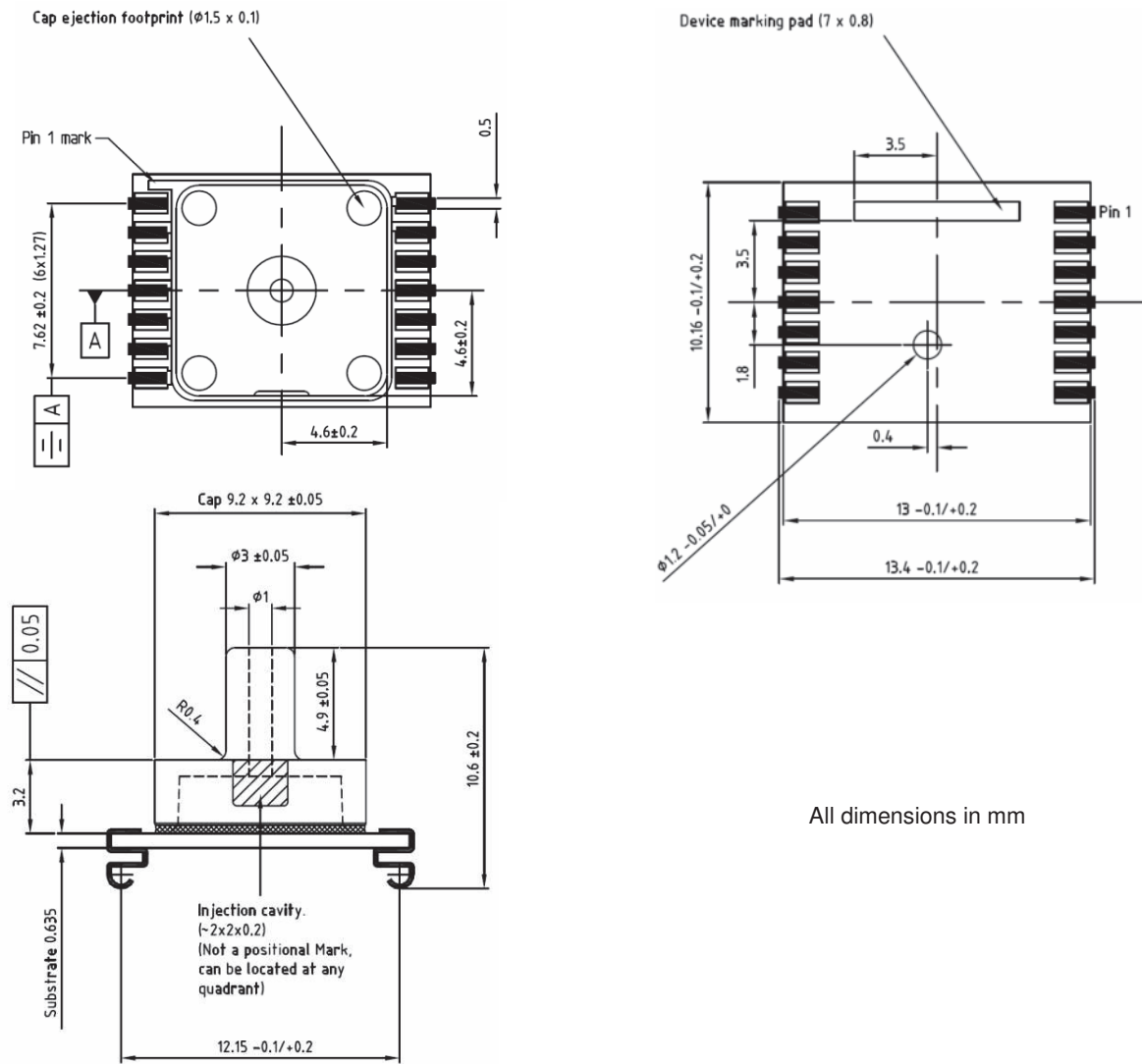
Fig. 8: Device package outlines of MS5536-CPJU / MS5536-CNJU
