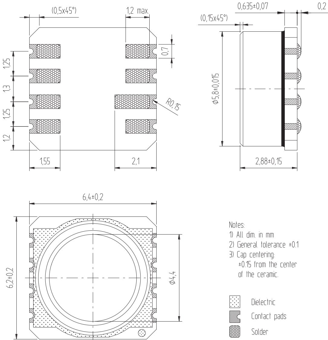
Fig. 8: Device package outlines of MS5541-C
