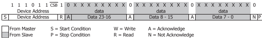
Figure 15: I 2 C answer from MS5607-02BA
